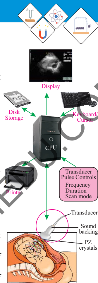
Fig: 11.14. The schematic diagram of the ultrasound scan machine
