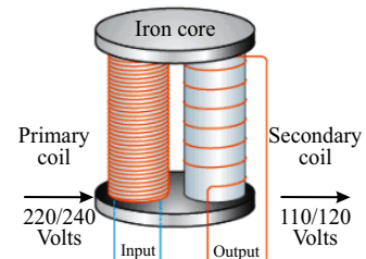
Fig: 16.18 (b) Step down transformer
