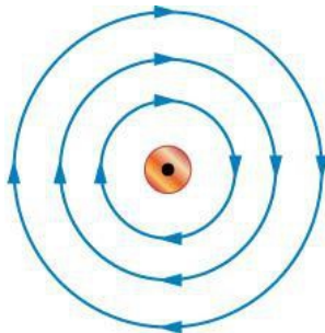
Fig: 16.5 Demonstration of the right-hand rule for conductors.
