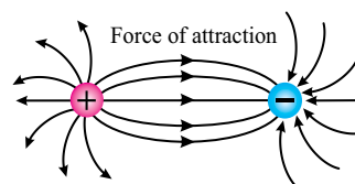
Fig: 14.11 (c) Two equal unlike charges
