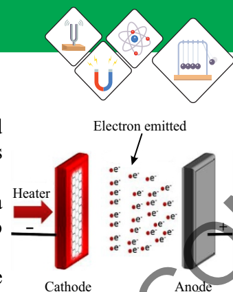
Fig: 17.12. Model for thermionic emission
