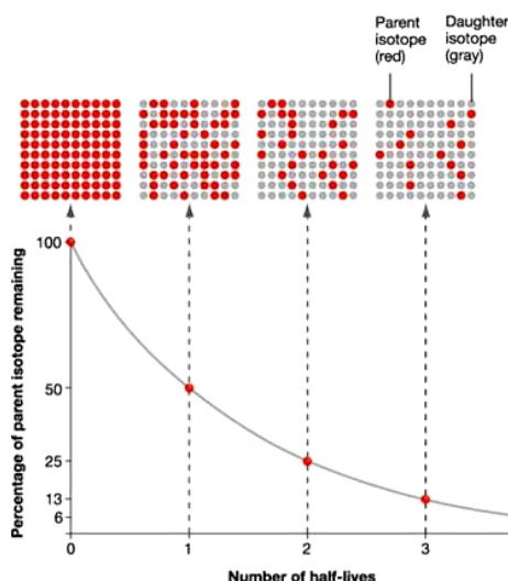
Fig: 20.8 Radioactivity of iodine
