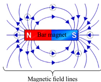
Fig: 16.8. Magnetic field lines
