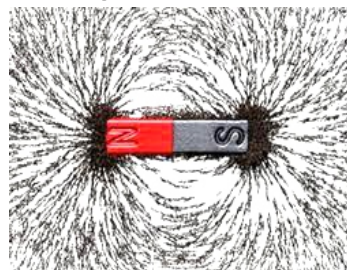
Fig: 16.8. Magnetic field lines
