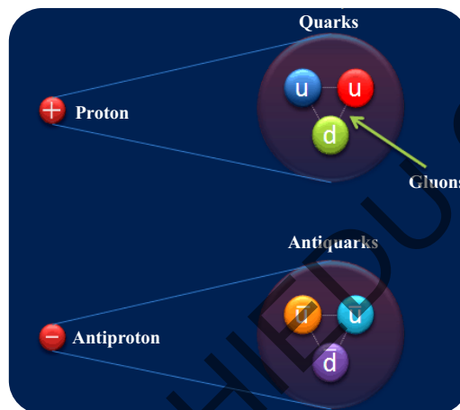
Fig: 19.5 The strong force binds quarks together in clusters to make more-familiar subatomic particles, such as protons and neutrons. It also holds together the atomic nucleus and underlies interactions between all particles containing quarks.
