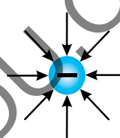
Fig: 14.11 (b) Isolated negative charge
