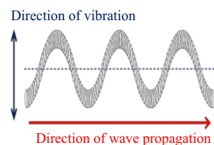
Fig: 10.6. A transverse wave in a slinky
