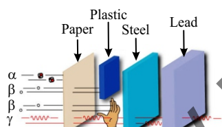
Fig: 20.4. Relative penetrating abilities of three kinds of radiations.
