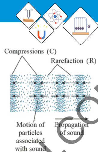
Fig. 11.2. The vibrating drum skin produce alternating regions with high density and low density of air molecules
