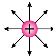
Fig: 14.11 (a) Isolated positive charge
