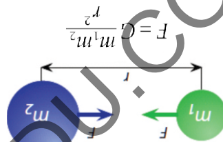
Fig (6.1) Newton's Law of Universal Gravitation
