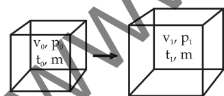
Fig (9.9) Volumetric expansion
