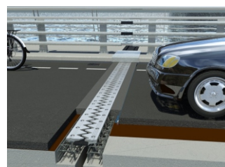
Fig (9.7) (c) Thermal expansion
