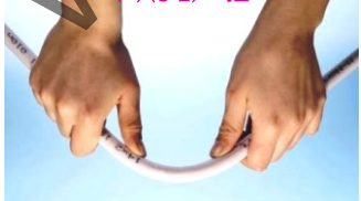
Fig (5.2)(a) A Force can bend an object
