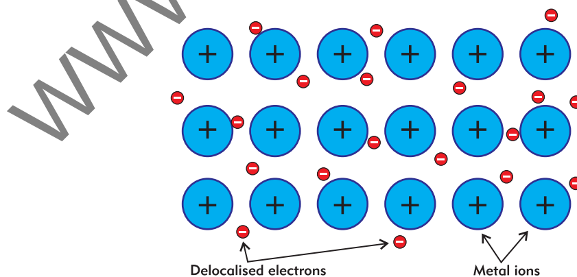
Fig 4.10 Diagrammatic representation of metallic bonding
