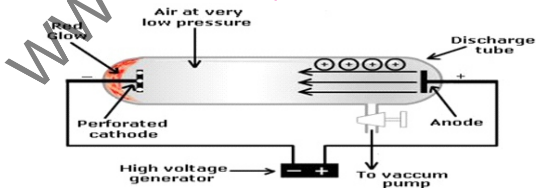
Fig 2.9 Gold Stein Discharge Tube
