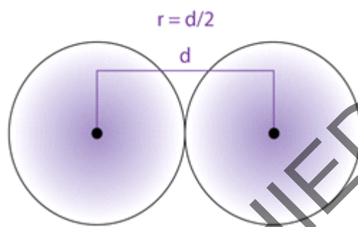
Fig 3.3 Atomic radius
