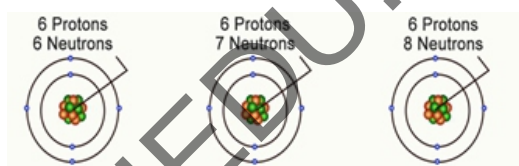
Fig 2.23 Isotopes of Carbon
