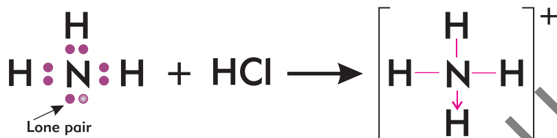
Fig 4.9 Reaction between Ammonia and Hydrogen Chloride
