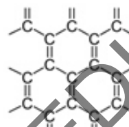
Fig 5.20 Graphene
