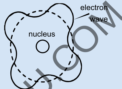
Fig 2.15 De Broglie wave duality hypothesis
