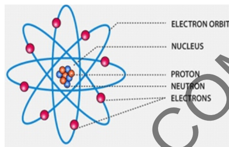
Fig 2.13 Rutherford Atomic Model
