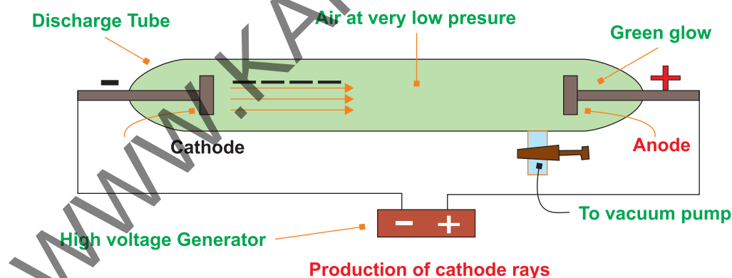
Fig 2.7 William Crookes Discharge Tube
