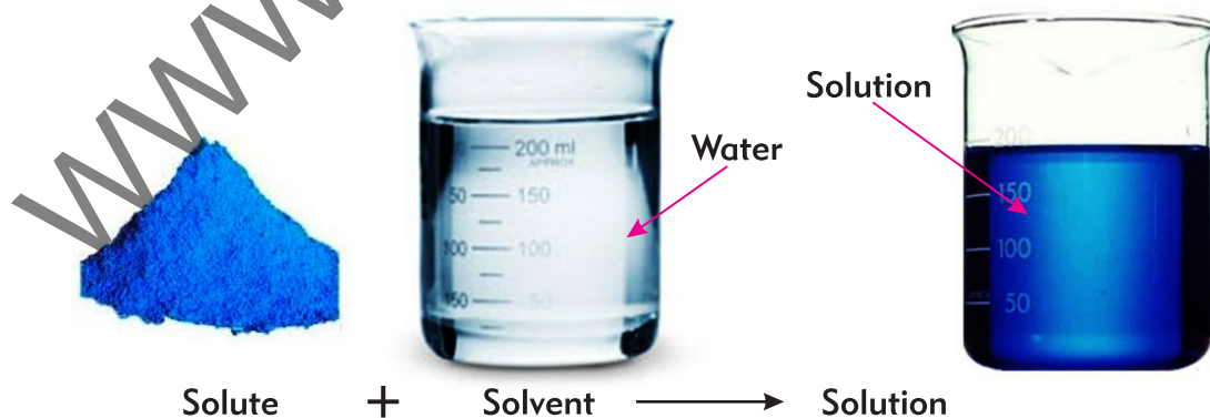
Figure 6.1 Preparation of Solution
