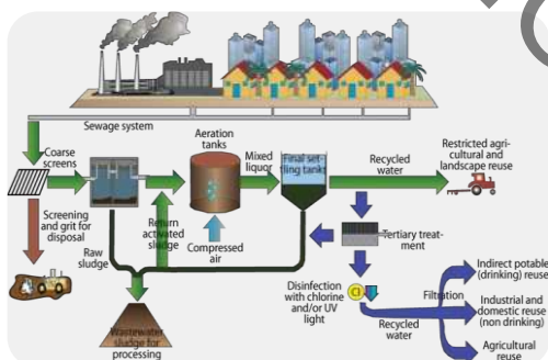
Fig. 7.28 Sewage Treatment
