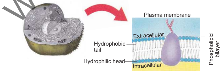
Figure 4.11 Cell membrane showing arrangement of phospholipid molecules in bilayers
