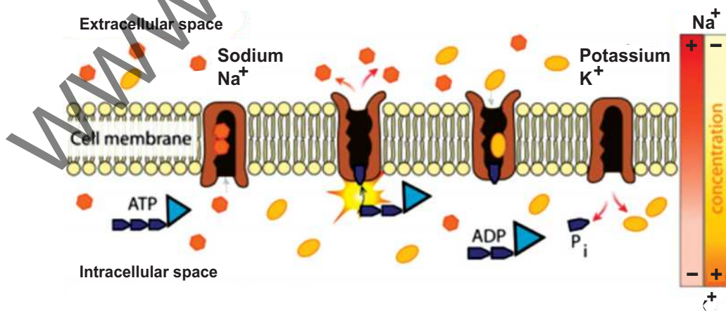
Figure 4.18 The sodium-potassium pump is an example of primary active transport.
