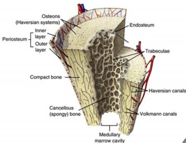
Figure 4.31 Longitudinal section of bone
