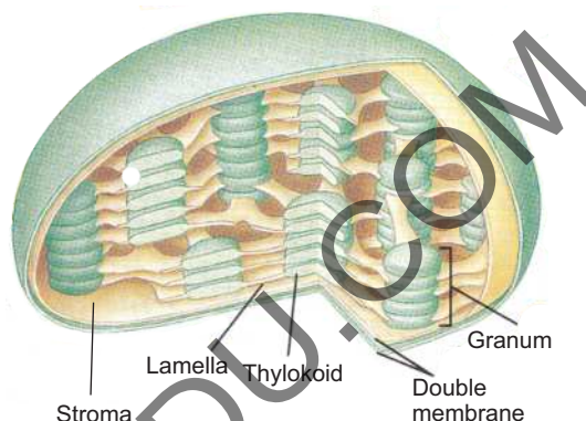
Figure 4.27 Structure of chloroplast
