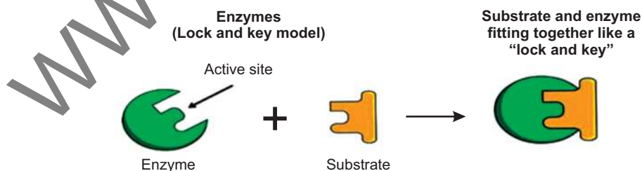
Figure 6.5 Lock and Key model
