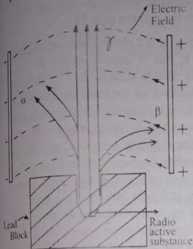
Fig.19.2 (a) Rutherford Experiment
