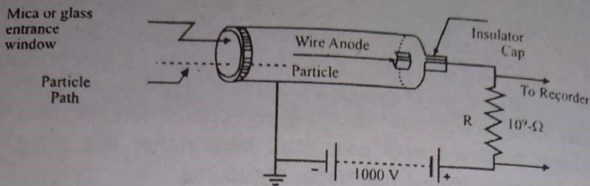
Fig.20.3 Geiger Counter
